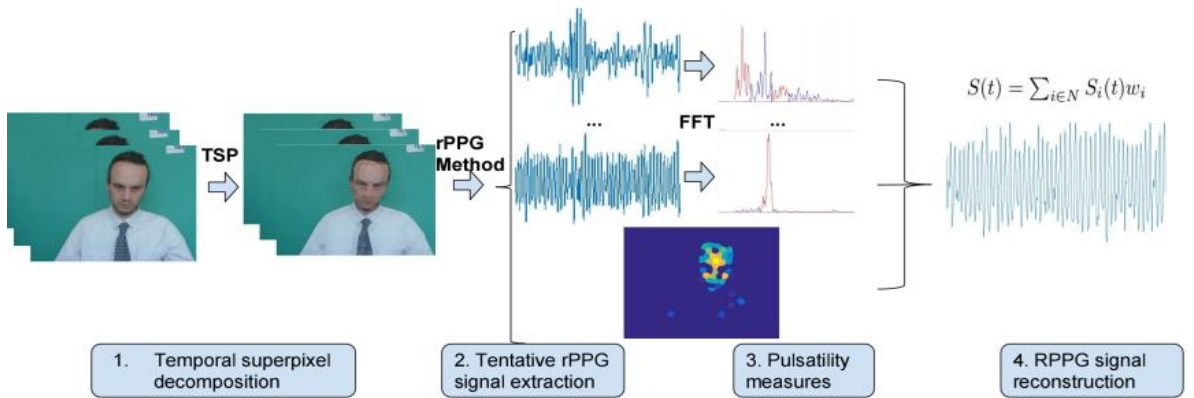
Figure 2.6 SNR-based region weighting method [15]
